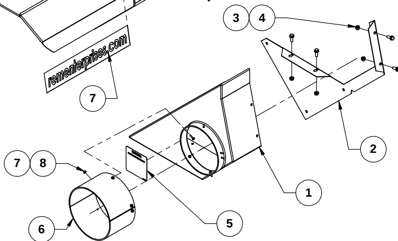
3700 LOWER FRONT GUARD ASSEMBLY PT #55-111191
