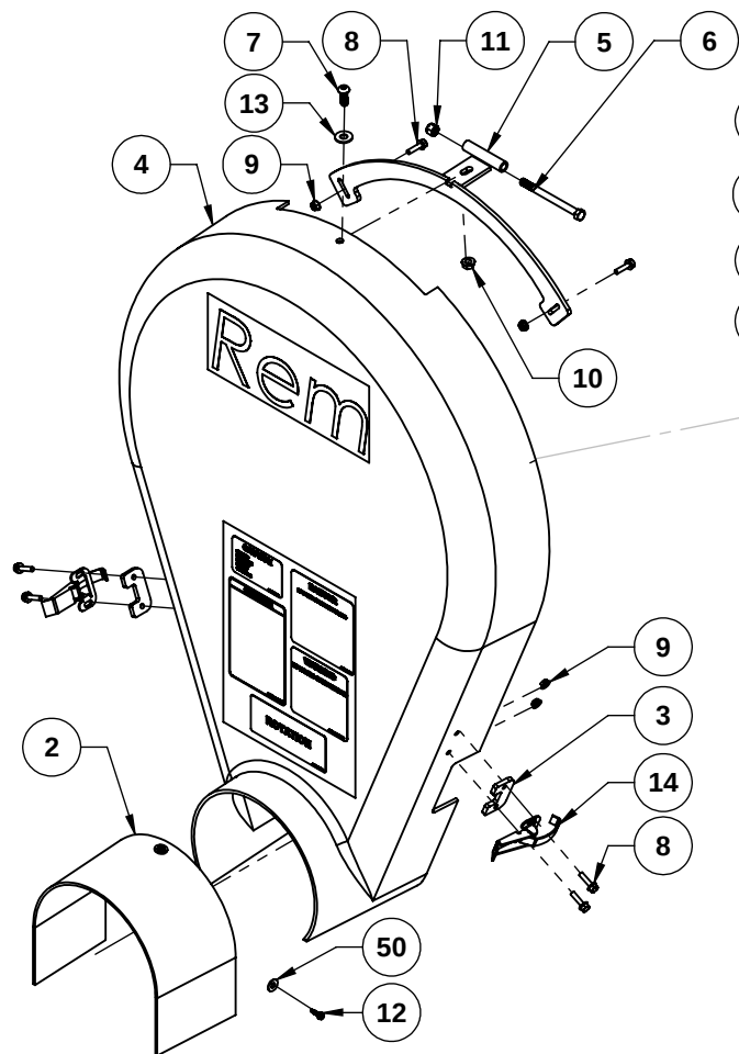
FRONT GUARD
